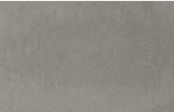
Iron
