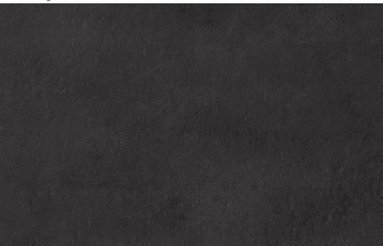
Graphite
